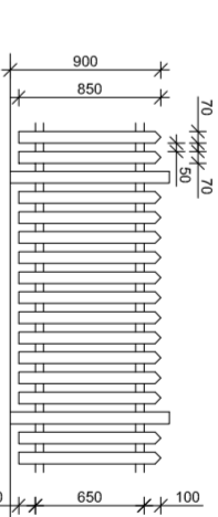
PICKET FENCE DETAIL SCALE 1:50
